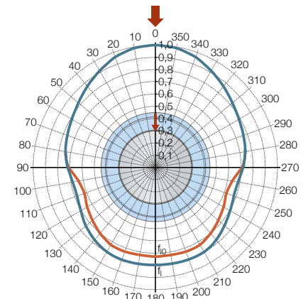
Diagram 13 Factors f_i and f_{i,0} related to the direction of load for LBCR and LBCD A-series linear ball bearings
