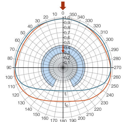
Diagram 15 Factor f_i and f_{i,0} related to the direction of load for LBHT linear ball bearings
