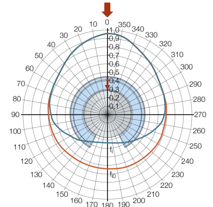
Diagram 14 Factor f_i and f_{i,0} related to the direction of load for LBCT and LBCF A-series linear ball bearings
