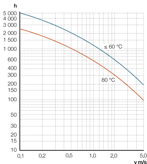
Relubrication interval
